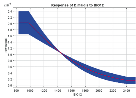
Figure 5. Relative occurrence rate (ROR) response curves of D. maidis concerning the model predictor variables: (A) BIO1 (B) BIO12 (C) BIO17 (D) ETo_annual (E) GSTD, and (F) Vv_annual. Source: Own elaboration.
